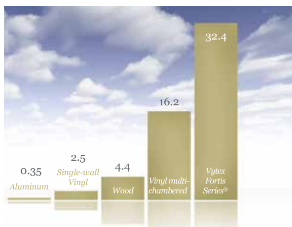
R-value for Window Frame Materials
