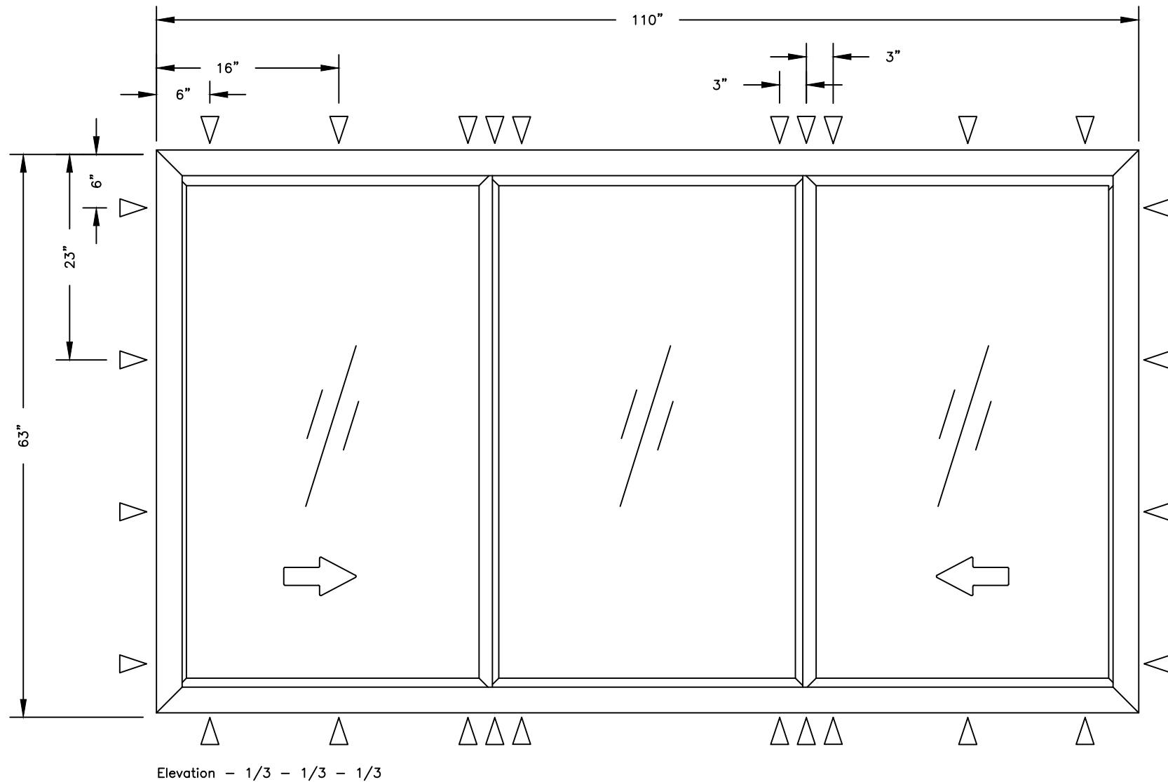
6200 HORIZONTAL SLIDING WINDOW (XOX) – FINLESS INSTALLATION MAXIMUM SIZE 110" X 63" DESIGN PRESSURE +/- 55 PSF (non-impact)
