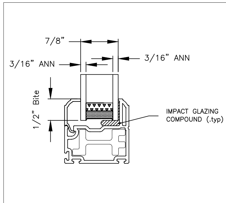
GLAZING DETAIL
