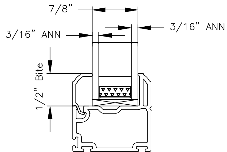
GLAZING DETAIL
