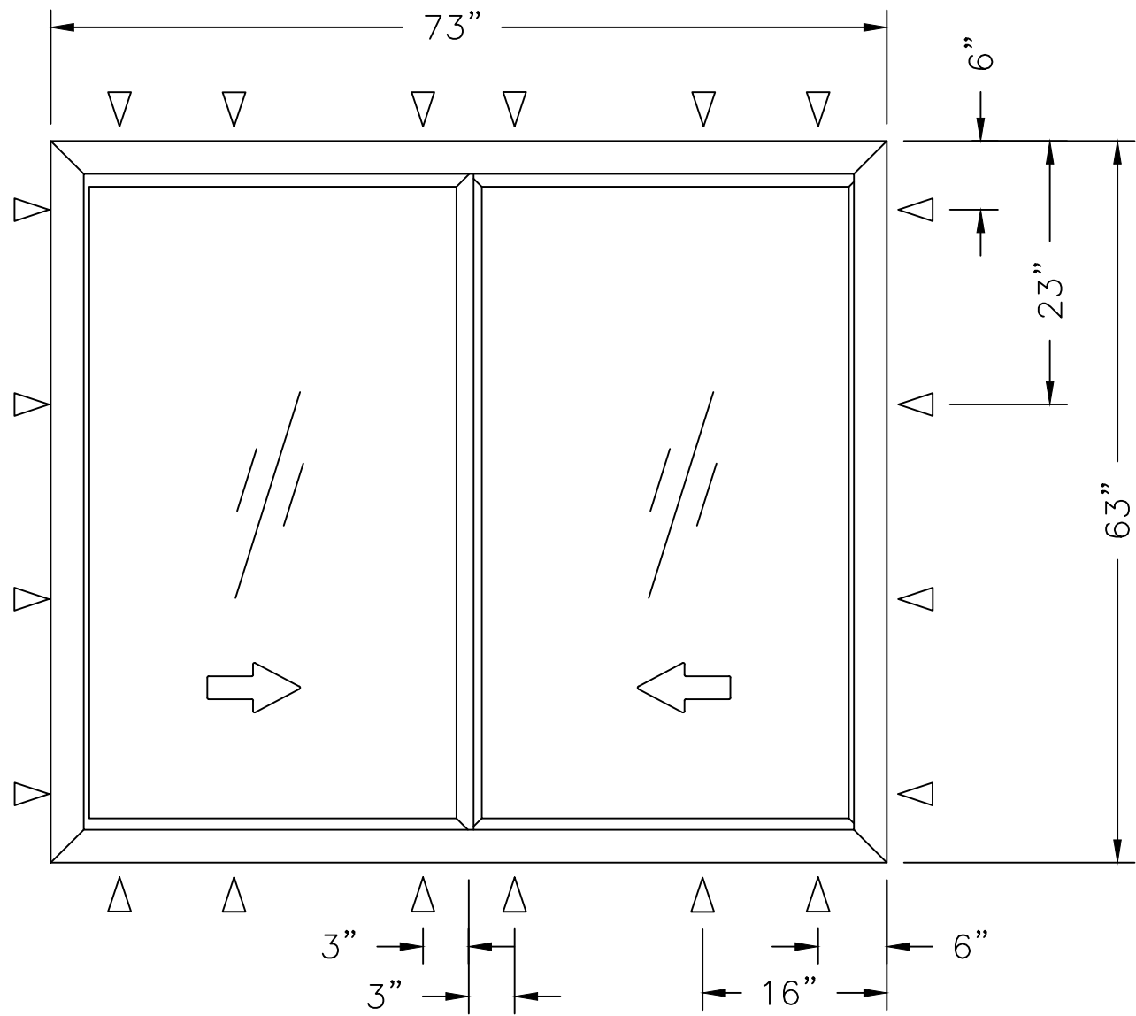
6000 HORIZONTAL SLIDING WINDOW (XX) – FINLESS INSTALLATION MAXIMUM SIZE 73" X 63" DESIGN PRESSURE +/- 55 PSF (non-impact)
